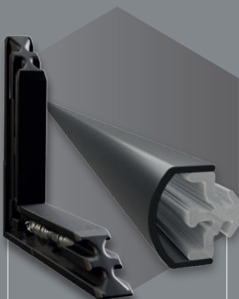
Features standard Prestige cleats, chevrons, gaskets and georgian bars for reduced stock holding
