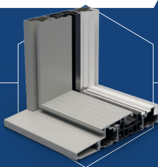
Standard Outer Frame with Clip-on Cill Nose
