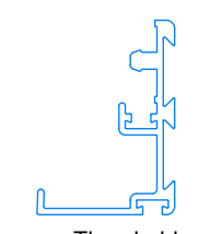
Threshold (White or Black) 704180 (A00180)
