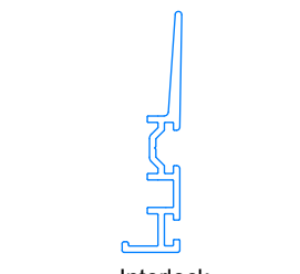
Interlock (White, Black or Foiled) 704181 (A00181)
