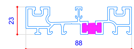
Patio Low Threshold (Silver or Gold) 104324
