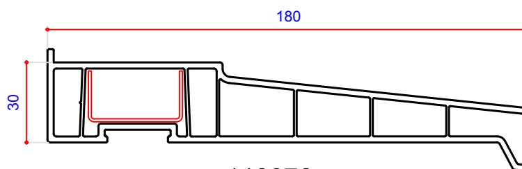
180mm Cill 110076 Steel U Channel 35 x 19mm 113377 End Cap 109090
