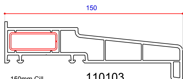
150mm Cill 110103 Steel Box 713016 (S00016) End Caps 109006 Straight Coupler 109010
