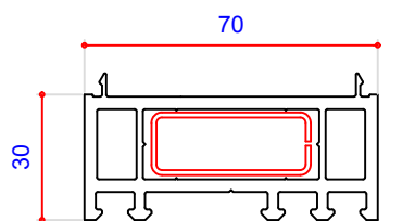
30mm Frame Extension 114014 Steel Box 38 x 15mm 113073
