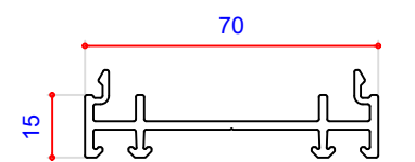
15mm Frame Extension 114037
