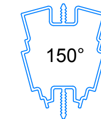
150° Bay Post 116065
