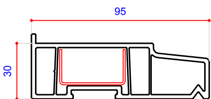
95mm Cill 110074 Steel U Channel 35 x 19mm 113377 End Cap 109074
