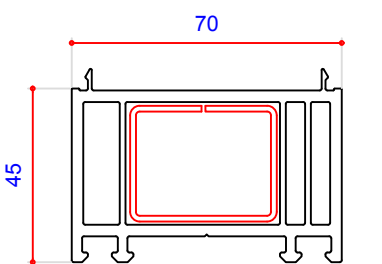
45mm Frame Extension 114202 Steel Box 38 x 30mm 113271
