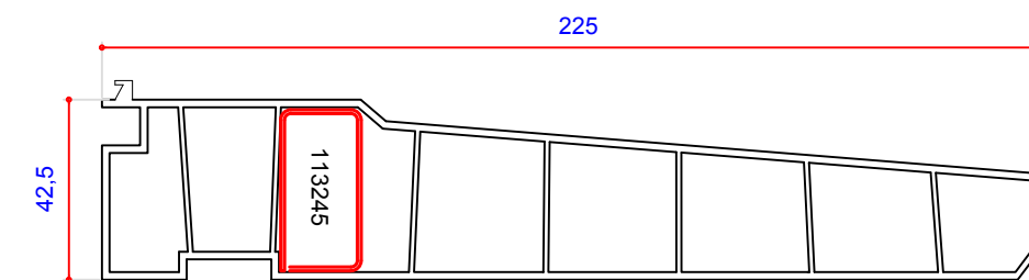
225mm Cill 110106 Steel Box 38 x 19 113245 Steel U Channel 38 x 19 113317 End Cap 109647
