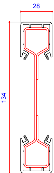
Dogbone Coupler 113112 Covering Profile 113073
