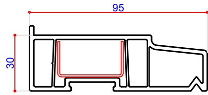
95mm Cill 110074 Steel U 35 x 19mm 113377 End Cap 109074
