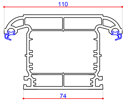
110mm Midrail 102264 Steel Box 113376 Aluminium Box 115286
