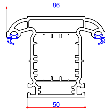
86mm T Mullion 102263 Steel Box 2.5mm 113378 Steel Box 1.2mm 113378 Steel P Section 113371
