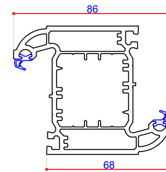
86mm Z Mullion 102262 Steel Box 2.5mm 113378 Steel Box 1.2mm 113378 Steel P Section 113371
