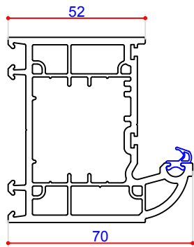
70mm Outer Frame 101228 Steel Box 2.5mm 113378 Steel Box 1.2mm 113378 Steel P Section 113371
