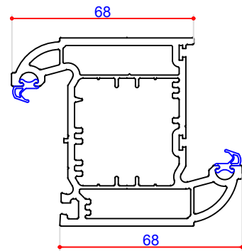
86mm Z Mullion 102303 Steel Box 2.5mm 113378 Steel Box 1.2mm 113378 Steel P Section 113371
