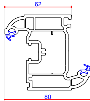
80mm Tilt & Turn Sash 103267 Steel L Section 113373 #LBH-X 8.5 x 32.5mm with No Steel
