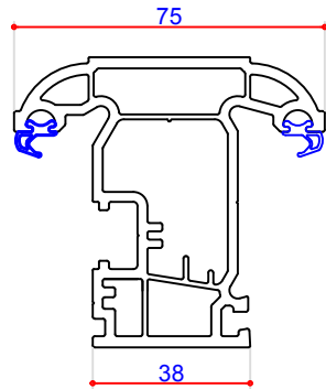
75mm Casement Sash 103264 Steel Box 113039 Steel P Section 113272 Steel Channel 113387
