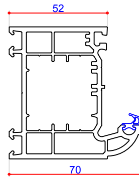
70mm Outer Frame 101161 Steel Box 2.5mm 113378 Steel Box 1.2mm 113378 Steel P Section 113371
