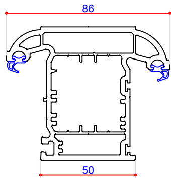
86mm T Mullion 102302 Steel Box 2.5mm 113378 Steel Box 1.2mm 113378 Steel P Section 113371
