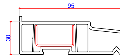
110074 95mm Cill Steel U 38 x 19 113377 End Caps 109074
