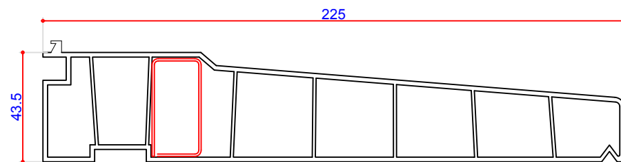
110106 225mm Cill Steel U Channel 38 x 19 113317 Steel Box 38 x 20 113245 End Caps 109647
