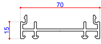
114037 15mm Frame Ext
