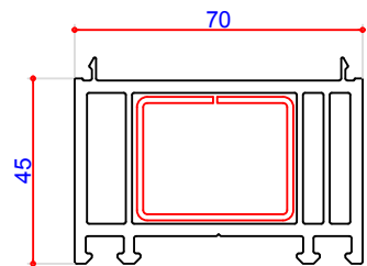
114202 45mm Frame Ext 38 x 30mm Steel Box 113271
