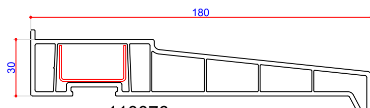
110076 180mm Cill Steel U Channel 38 x 19 113377 End Caps 109090
