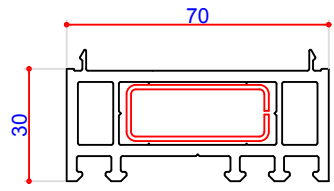
114014 30mm Frame Ext 38 x 15mm Steel Box 113073
