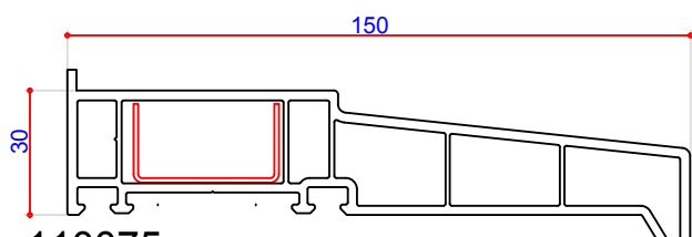
110075 150mm Cill Steel U Channel 113377 Steel Box 38 x 20 113245 Straight Joint 109085 135° Joint 109084 90° Joint 109089 End Cap 109075
