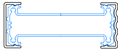
115117 20mm Aluminium Coupling Plain Cover 716323 Sculptured Cover 716324
