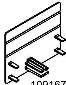
109167 Profile Cover Cap
