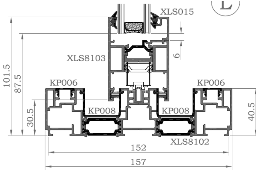
Triple Track Threshold Schematic
