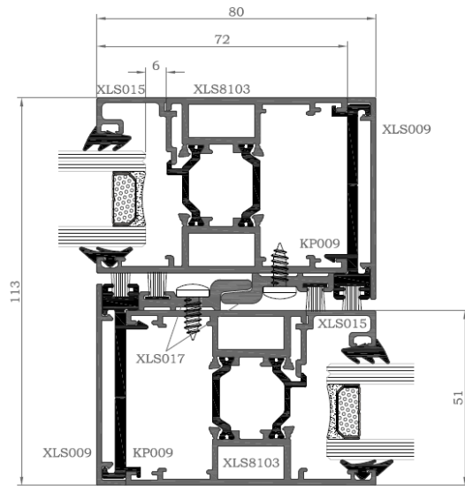
Interlock Details
