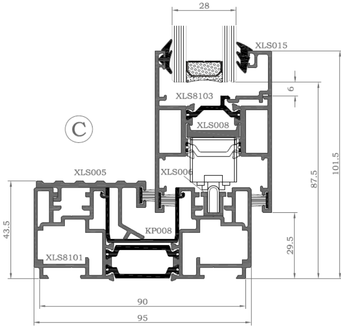
Double Track Threshold Schematic
